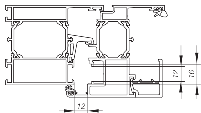
Screw plate for 16 mm fittings groove
