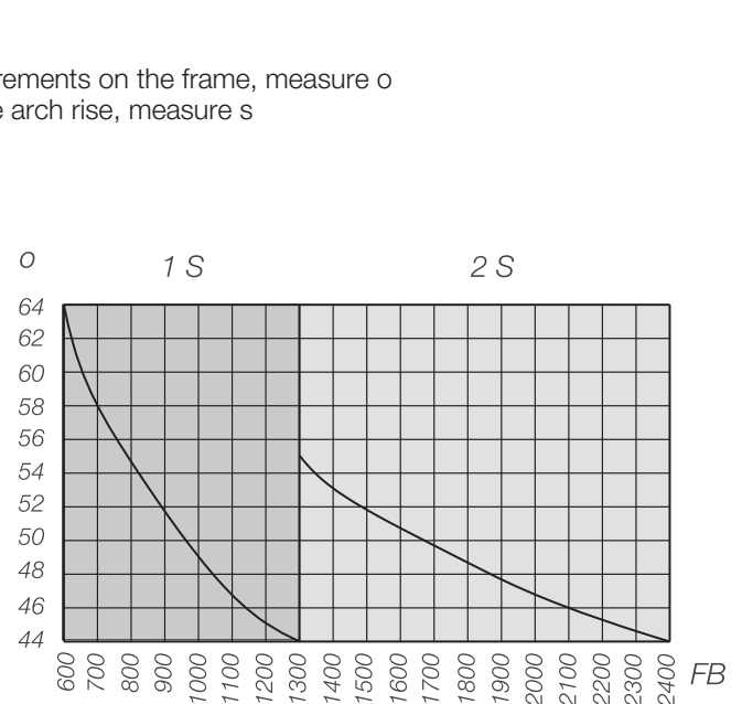
Round arch window
