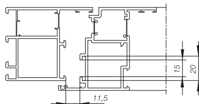
Clamping plate for Alu fittings groove 15/20
