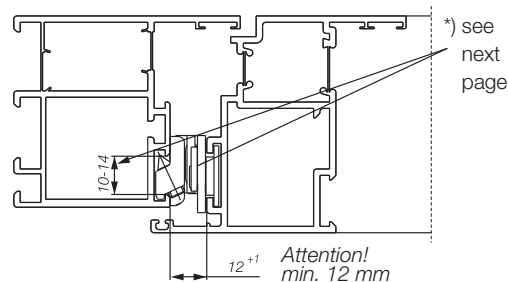
Vertical section KSP on the aluminium window
