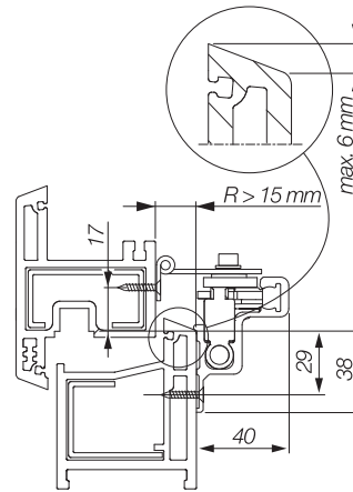
Vertical section on the PVC window with stay holder 2
