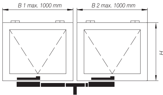
PRIMAT-A, type: hm, 2 sashes, side-by-side
